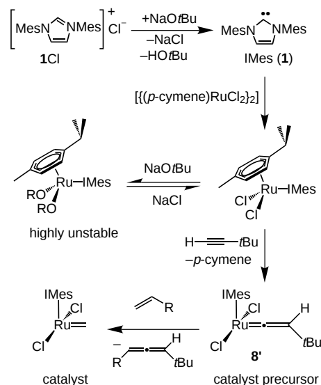
Scheme 1. Proposed pathways for catalyst generation and decomposition.
